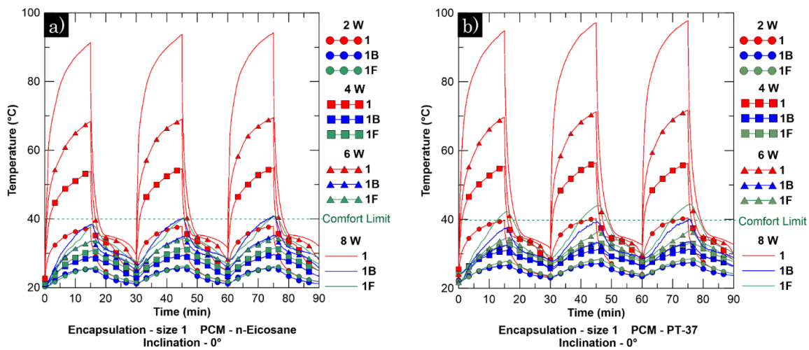
Figure 10. Influence of power input levels on the thermal response of the experimental tablet PC at 0° inclination with Size 1 PCM TES unit: (a) n -eicosane and (b) PT-37.
