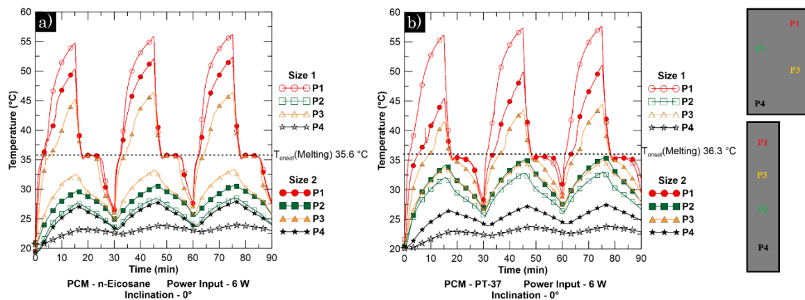
Figure 6. Influence of PCM TES size on PCM melting at 6 W power input and 0° inclination: (a) n -eicosane and (b) PT-37.
