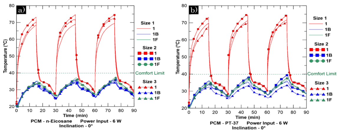
Figure 11. Influence of PCM TES size on the thermal response of the experimental tablet PC at 6 W power input and 0° inclination: (a) n -eicosane and (b) PT-37.
