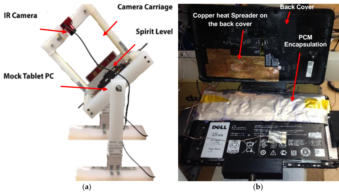
Figure 1. Photograph of the experimental setup showing (a) the inclined test stand and (b) the mock tablet PC with Size 2 PCM (phase change material) encapsulation on display. IR: Infrared.
