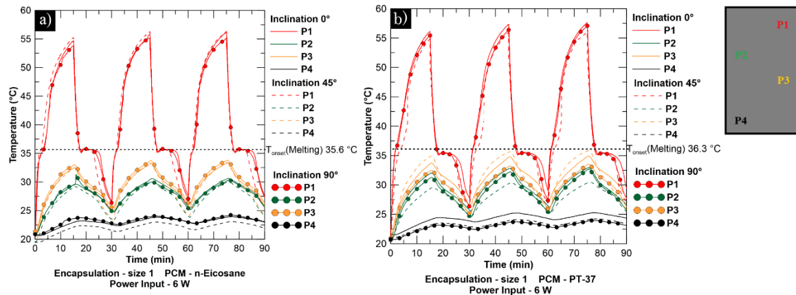
Figure 4. Influence of inclination on PCM melting for intermittent operation at 6 W power input with Size 1 PCM TES Unit: (a) n -eicosane and (b) PT-37.
