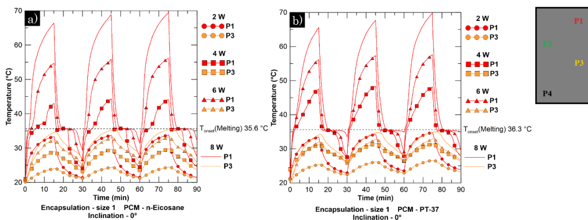
Figure 5. Influence of power input levels on PCM melting for intermittent operation at 0° inclination with Size 1 PCM TES Unit: (a) n -eicosane and (b) PT-37.
