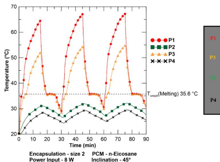
Figure 3. Melting curves of n -eicosane for Size 2 TES unit at 45° inclination and 8 W power input.
