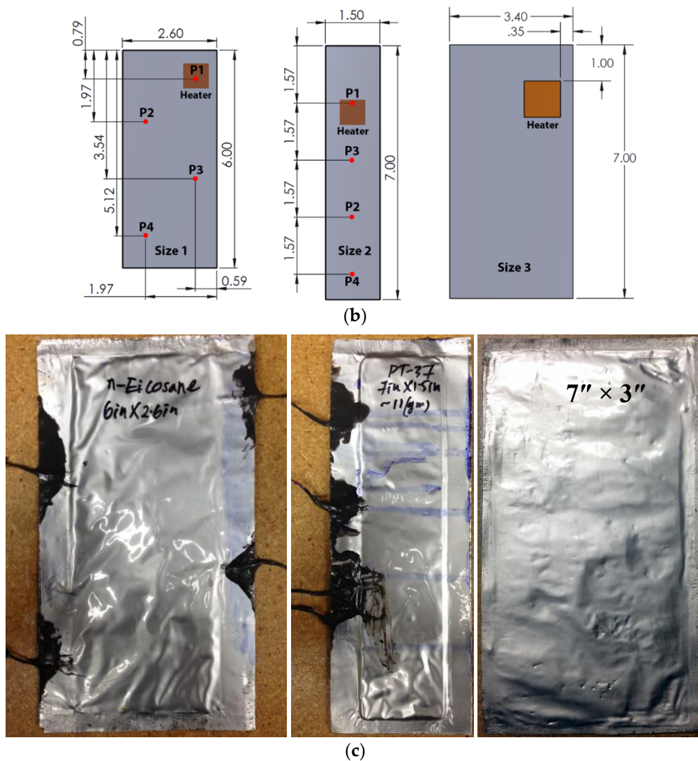
Figure 2. (a) Positions of thermocouples attached to internal components and to front and back surfaces of the mock tablet PC (F—Front, B—Back), (b) schematics of the three different sized encapsulations with positions of thermocouples relative to the tablet PC heater (dimensions in inches) (c) photographs of PCM encapsulations: Size 1 (Left), Size 2 (middle), Size 3 (right).
