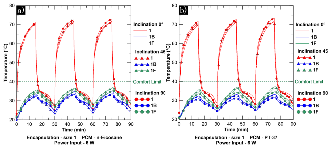
Figure 9. Influence of inclination on the thermal response of the experimental tablet PC at 6 W power input with Size 1 PCM TES Unit: (a) n -eicosane and (b) PT-37.
