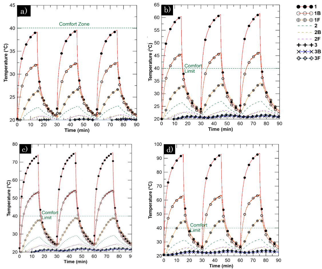
Figure 7. The baseline temperature profile for the experimental tablet PC at various power input without any PCM TES units: (a) 2 W, (b) 4 W, (c) 6 W and (d) 8 W.
